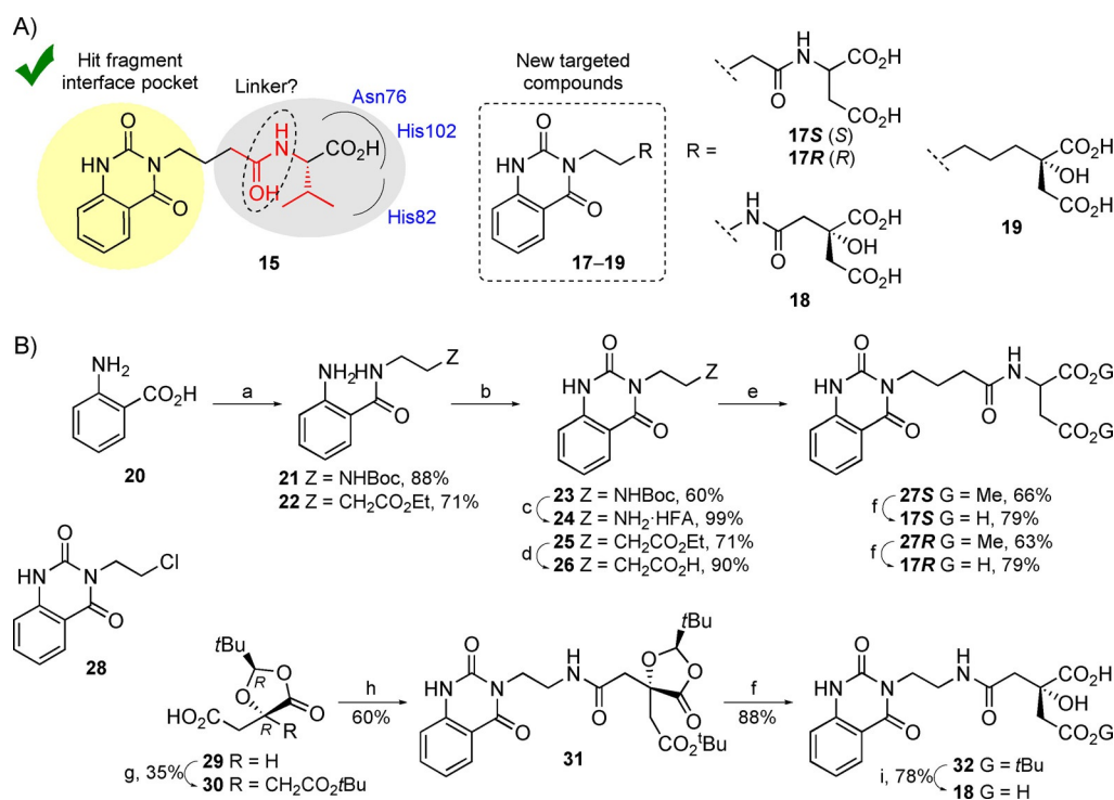
Figure 5. A) Explored chemical modifications of the carboxylate containing chain in 15 , and new targeted quinazolinone derivatives 17–19 . B) Synthesis of compounds 17S , 17R and 18 . Reagents and conditions: a) N -Boc-ethylenediamine (for 21 ) or ethyl 4-aminobutanoate (for 22 ), EDC, DMAP, DMF, RT; b) triphosgene, DIPEA, CH 2 Cl 2 , RT; c) TFA, CH 2 Cl 2 , 0 °C; d) 1. LiOH, THF, RT, 2. HCl (10%); e) 1. SOCl 2 , 60 °C, 2. dimethyl L -aspartate (for 27S ) or dimethyl D -aspartate (for 27R ), Et 3 N, CH 2 Cl 2 , RT; f) 1. LiOH, 2. Amberlite IR-120 (H + ); g) 1. LHMDS, THF, –78 °C, 2. BrCH 2 CO 2 tBu, –23 °C; h) 24 , HATU, DIPEA, DMF, RT; i) HCl (4.5 M), RT.
