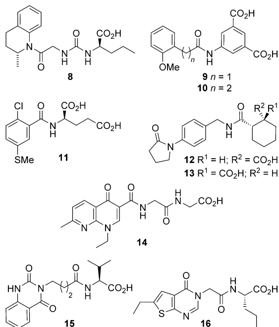
Figure 3. Selected potential inhibitors of the Hp -DHQ2 enzyme obtained by the fragment-based approach.
