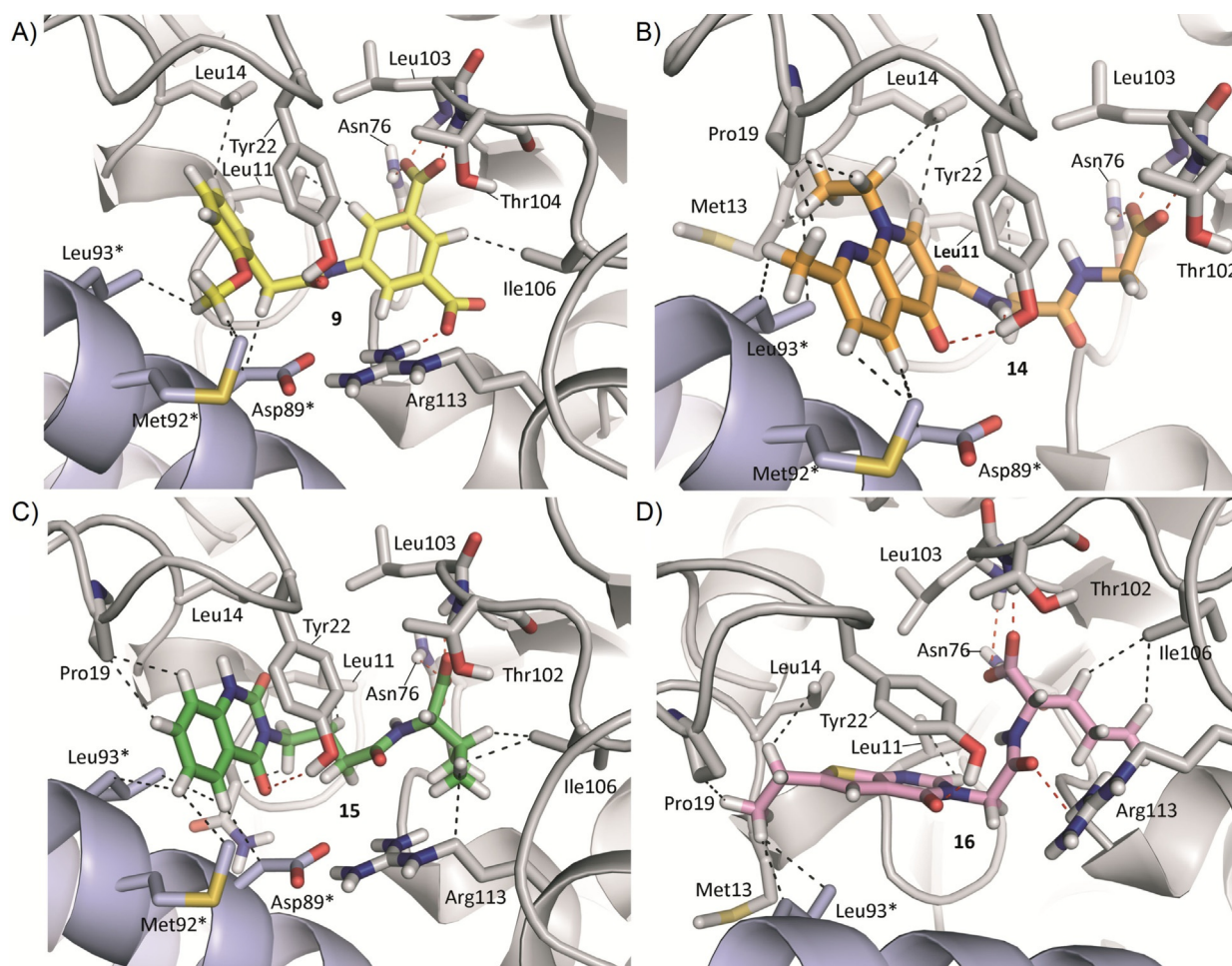
Figure 4. Selected view of the predicted binding mode of ligands: A) 9 (yellow), B) 14 (orange), C) 15 (green), and D) 16 (pink) in the Hp -DHQ2 active site. The neighboring chain close to the active site is shown in blue and its relevant side chain residues are indicated with an asterisk. Relevant side chain residues are shown and labeled. Hydrogen-bonding (red) and lipophilic (grey) interactions are indicated as dashed lines.
