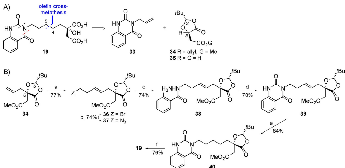
Scheme 1. A) Explored olefin cross-metathesis strategy for the synthesis of 19 . B) Synthesis of compound 19 . Reagents and conditions: a) 4-bromobutene, Grubbs–Hoveyda 2nd-generation catalyst, PhMe, 90 °C; b) NaN 3 , DMF, 90 °C; c) 1. Ph 3 P, THF, H 2 O, Δ, 2. 20, EDC, DMAP, RT; d) triphosgene, Et 3 N, CH 2 Cl 2 , RT; e) H 2 , Pd/C (10%), EtOH, RT; f) 1. LiOH, 2. Amberlite IR-120 (H + ).
