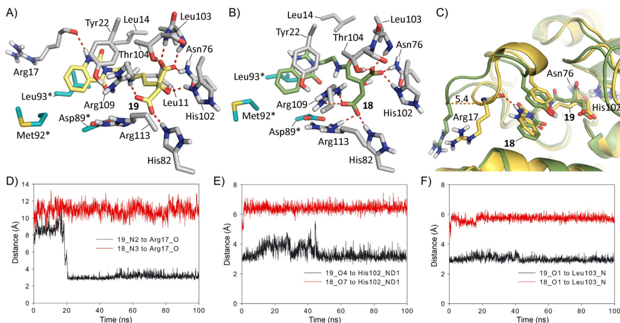
Figure 6. Detailed view of the predicted binding of ligands 19 (A, yellow) and 18 (B, green) in the active site of Hp -DHQ2 obtained by MD simulation studies. Both poses showed correspond to snapshots after 60 ns of MD simulation. Hydrogen-bonding interactions between ligand and several residues of the active site are shown as red dashes. C) Comparison of the binding mode of ligands 19 and 18 in the active site of Hp -DHQ2. D)–F) Variation of the relative distance between residues Arg117 (O atom, D), His102 (N \delta 1 atom, E), and Leu103 (N atom, F) and NH group of the aromatic moiety (N2 and N3 atoms), the medium chain carboxylate (O4, O7 and O1 atoms) in 19 and 18 , respectively, during the whole simulation. Note how ligand 19 has stronger hydrogen bonding interactions with the latter residues than ligand 18 and provides a closer and more organized conformation of the substrate-covering loop. Side chain residues from the neighbor chain are shown in cyan and labeled with an asterisk.
