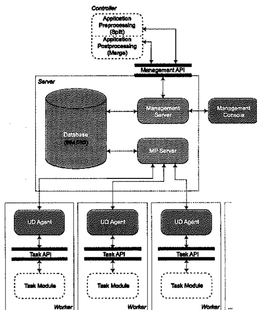
Figure 1: MetaProcessor platform overview.
